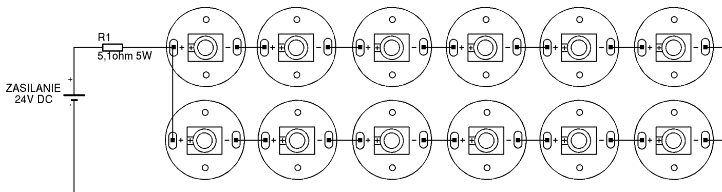
Fig. 5. Parallel connection of m-LUMO XR modules, drive voltage 24 V.
