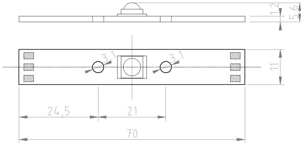
Fig. 1. MEGA 1XR module – basic version.
