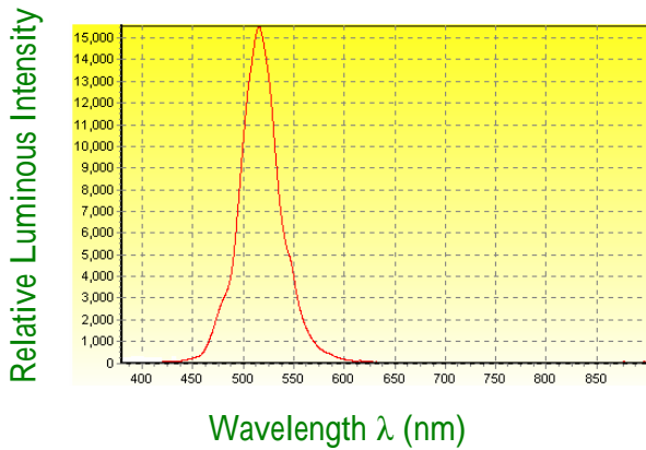
Wavelength Characteristics (Ta=25 )
