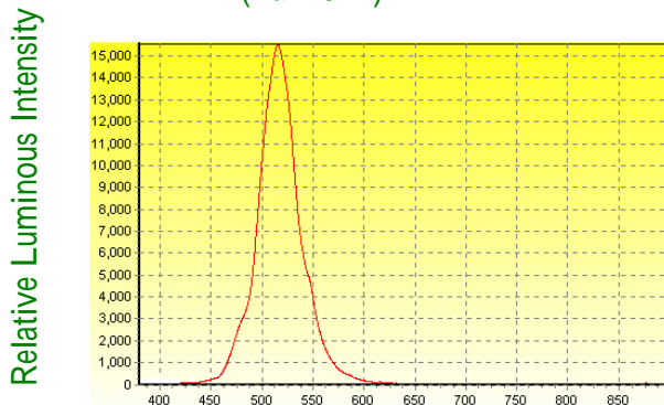
Wavelength Characteristics (Ta=25 )
