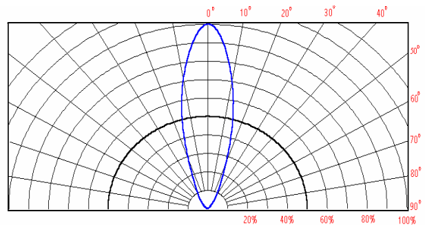
Directive Characteristics ( Ta=25 )
