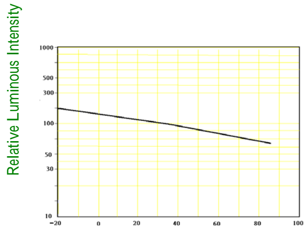
Ambient Temperature Ta ( )
