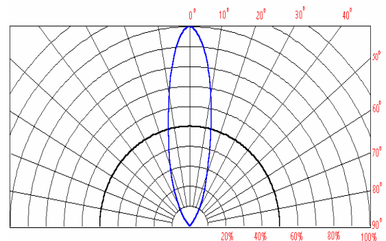
Directive Characteristics ( Ta=25 )
